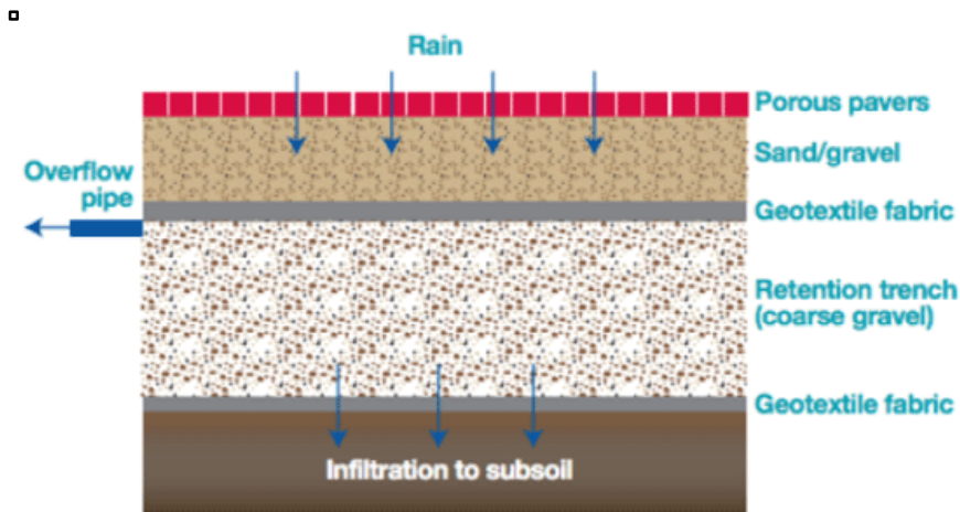
Figure 1: Schematic of porous asphalt and the infiltration of stormwater into subsoil. 67
