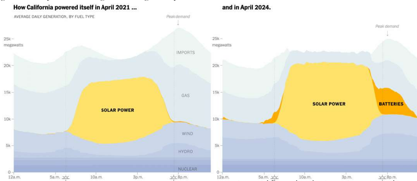
Figure 1: California's Change in Average Daily Generation
