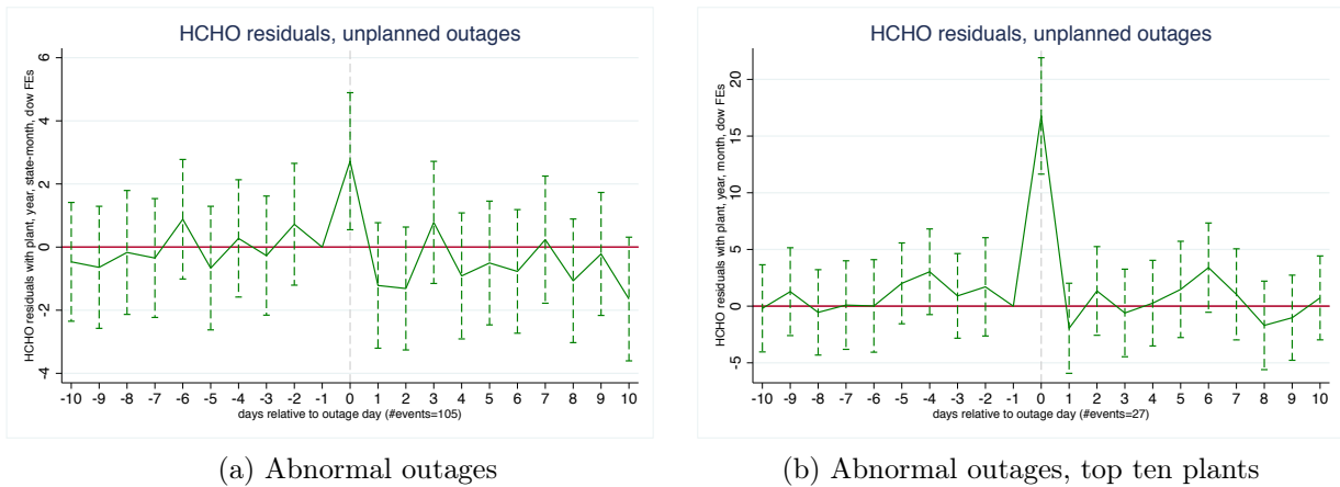
Figure 2: Effects of abnormal outages on surrounding HCHO
